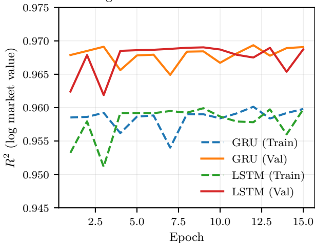
Training and validation R^2 : GRU vs LSTM
